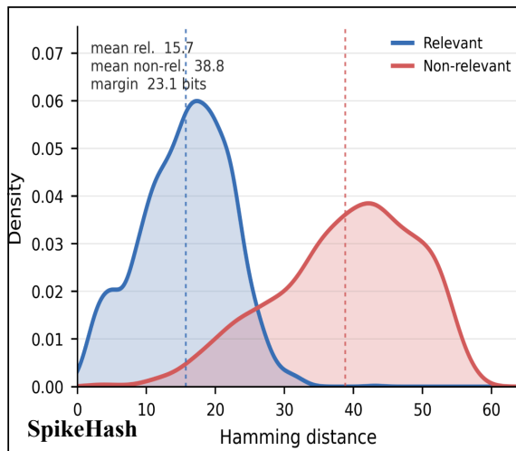
(b) Hamming distance distribution of positive and negative correlations
