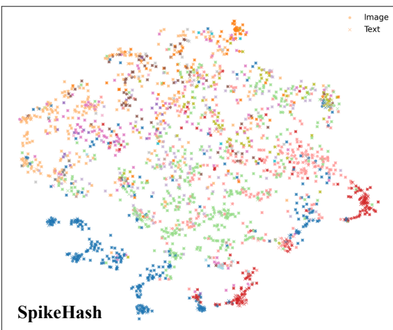
(a) Multi-label t-SNE distribution
